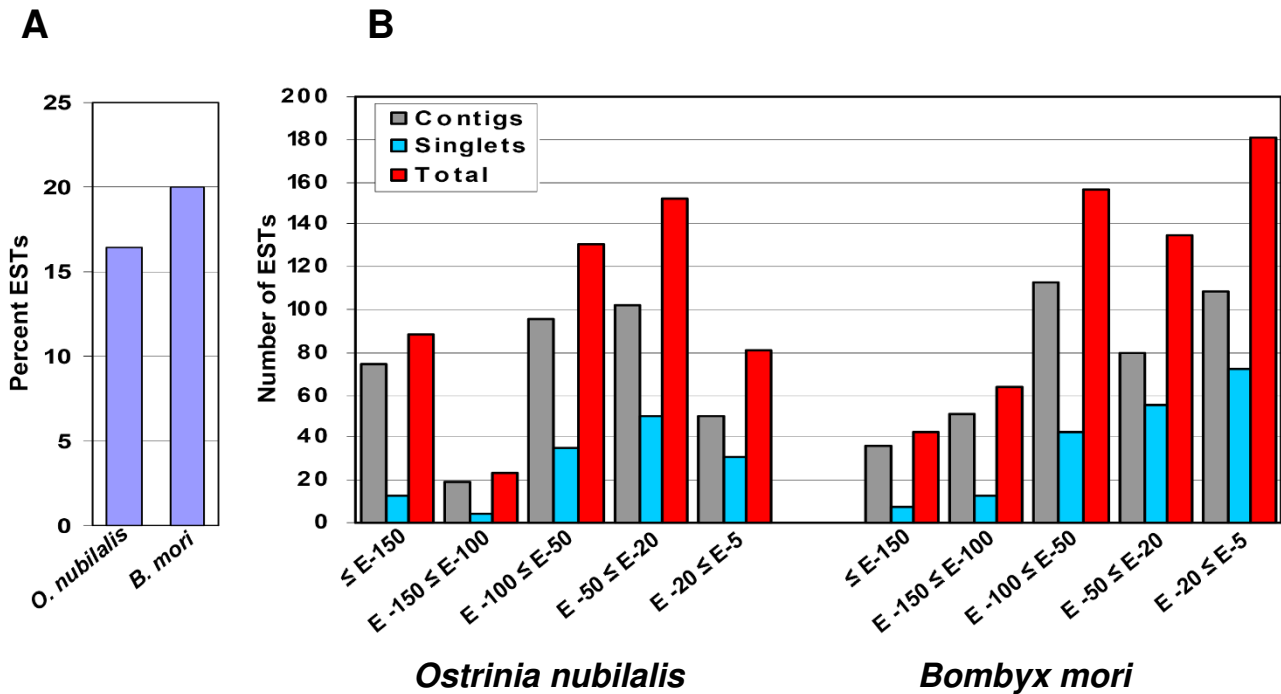
Figure 4 (A) Percentage of the 2,895 ECB gut-specific unique ESTs which shared matches with O. nubilalis and B. mori sequences with E-value ranging from E-150 to E-5 using BLASTN. (B) Comparative analyses of the 2,895 ECB gut-specific unique ESTs to B. mori sequences and other O. nubilalis sequences available in NCBI database using BLASTN.
