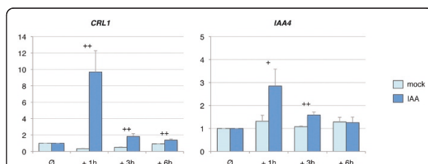
Figure 4 CRL1 expression is induced by auxin within 1 hour. Time course of transcription of CRL1 and IAA4 genes in response to mock or IAA treatment (0, 1, 3 or 6 hours) in WT and crl1 mutant assayed by RT-qPCR. Y-axis indicates the relative expression level at each timepoint relative to timepoint "0" (before treatment). IAA4 : early-auxin responsive gene, control of IAA treatment. h, hour after treatment. Values represent the mean obtained from 3 independent auxin treatment experiments, bars represent the standard deviation. Mean values were compared between WT and crl1 mutant for each time point. A significant difference was noted with one (p-value < 0.1) or two plus signs (p-value < 0.05).
