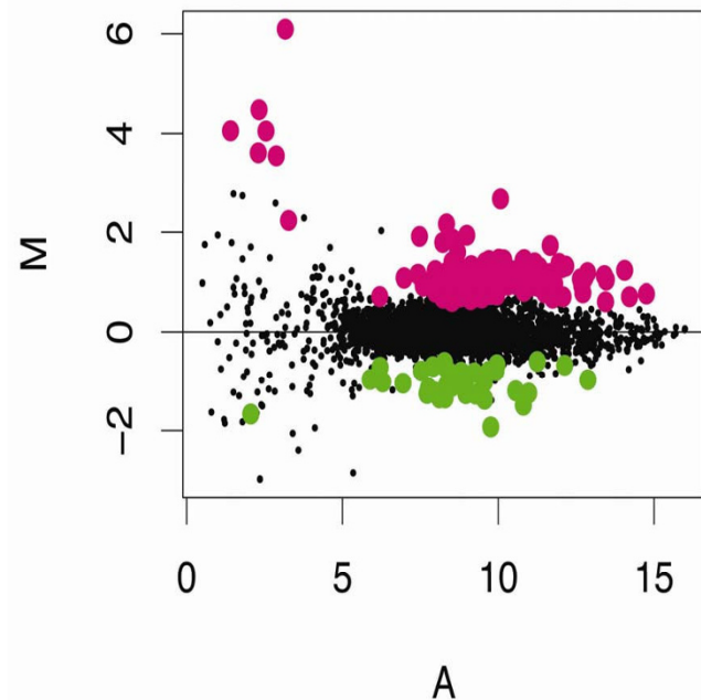
Figure 3 Cadmium effects on gene expression: Regulated genes. Gene expression data from control and cadmium (20 µg Cd/L for 48-h) treated Daphnia pulex [GEO:GSE9746]. Micorarray elements determined to significantly different ( p \leq 0.05 ) using the empirical Bayes (ebayes) method to shrink gene-wise error estimate in cadmium treated vs. control animals are highlighted (up-regulated elements in pink; down-regulated elements in green).
